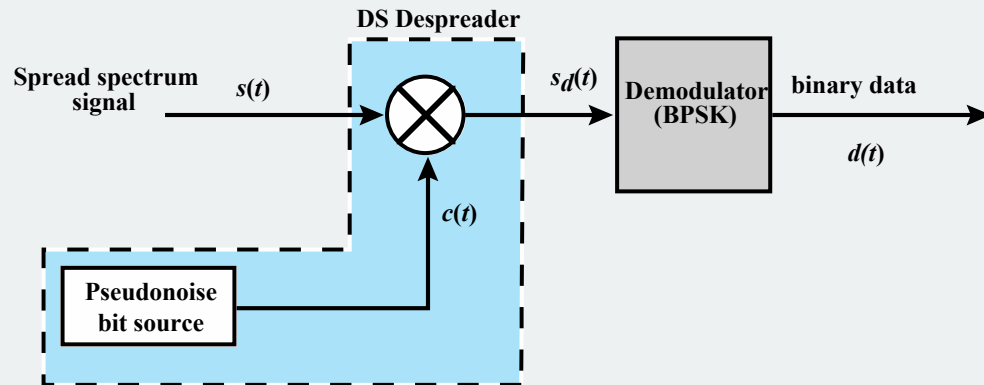
(b) Receiver
