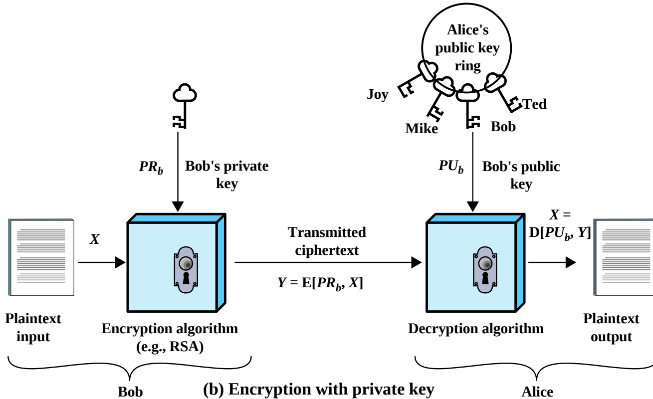
Figure 2.6 Public-Key Cryptography
